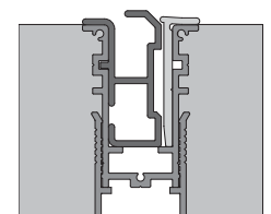
Flush track
